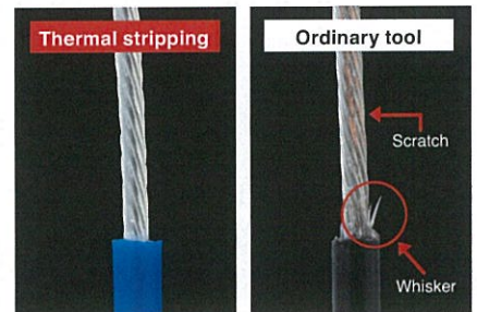
With a thermal wire stripper you can remove insulation cleanly without scratching core wires.
